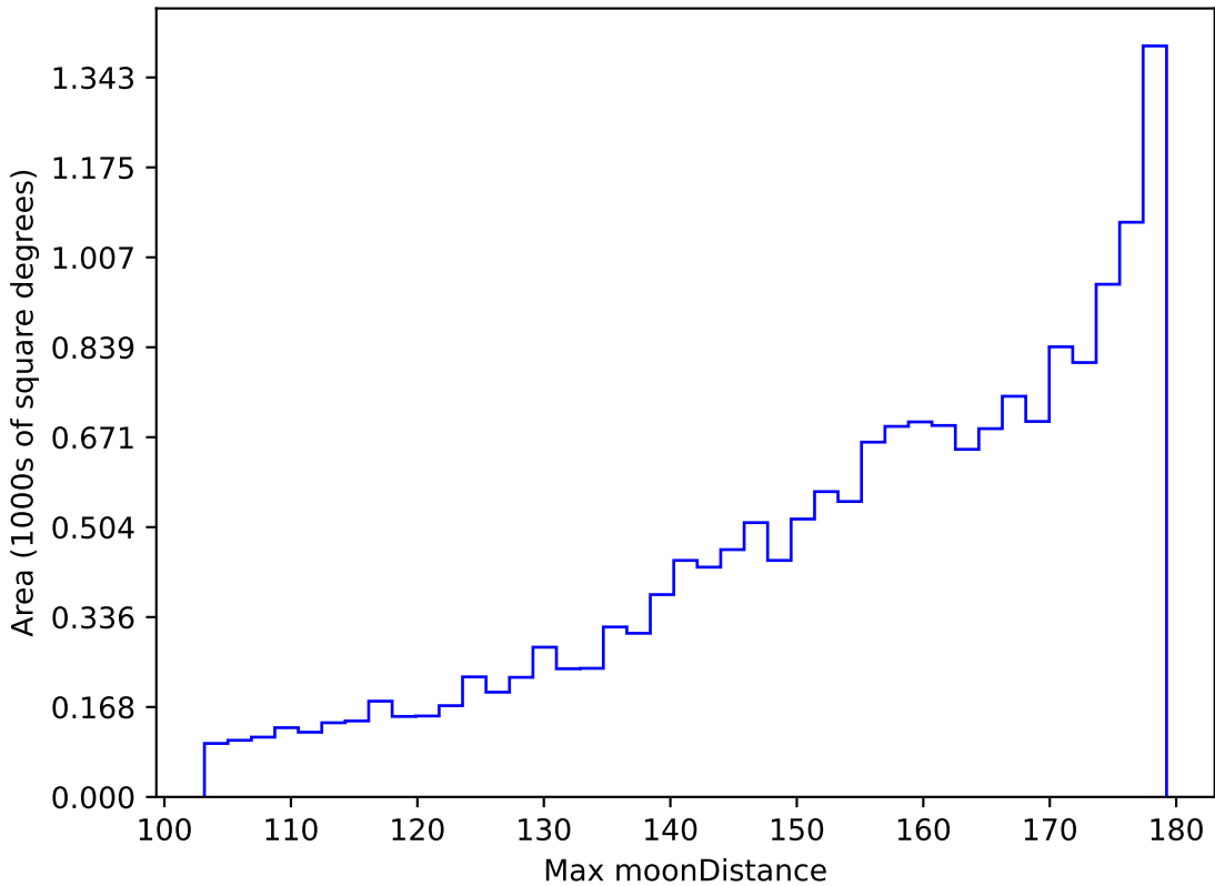
weather_cloudso0v3.4_10yrs WFD i band: Max moonDistance
