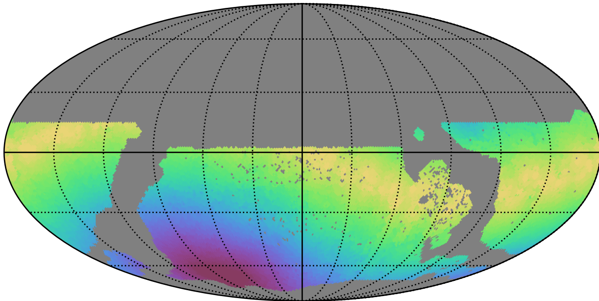
weather_cloudso0v3.4_10yrs WFD g band: Max moonDistance
