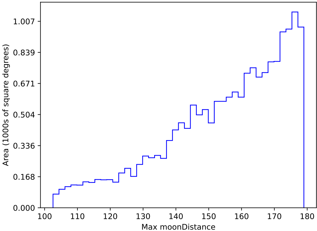
weather_cloudso0v3.4_10yrs WFD g band: Max moonDistance
