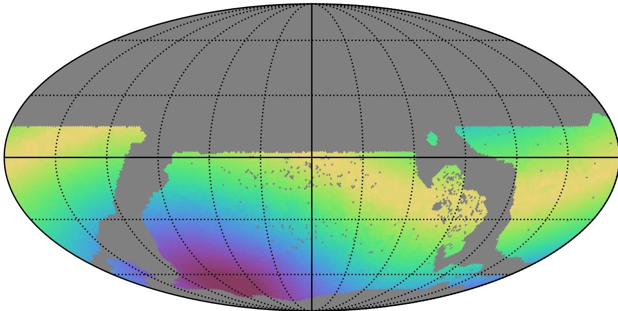
weather_cloudso0v3.4_10yrs WFD all bands: Max moonDistance
