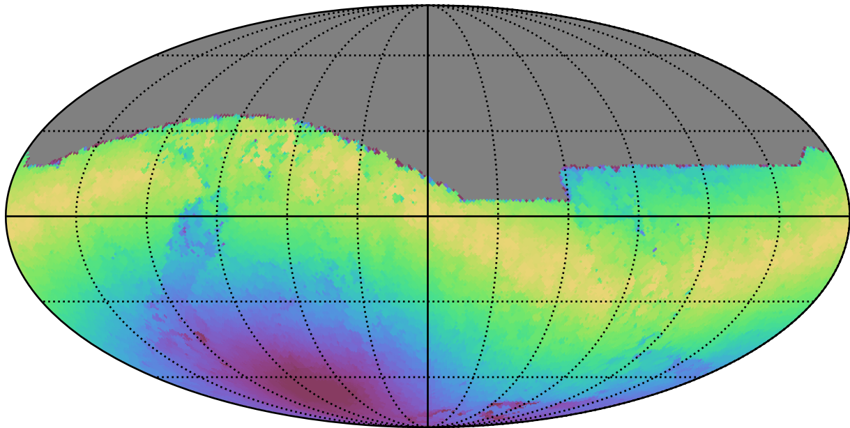
weather_cloudso0v3.4_10yrs All sky z band: Max moonDistance
