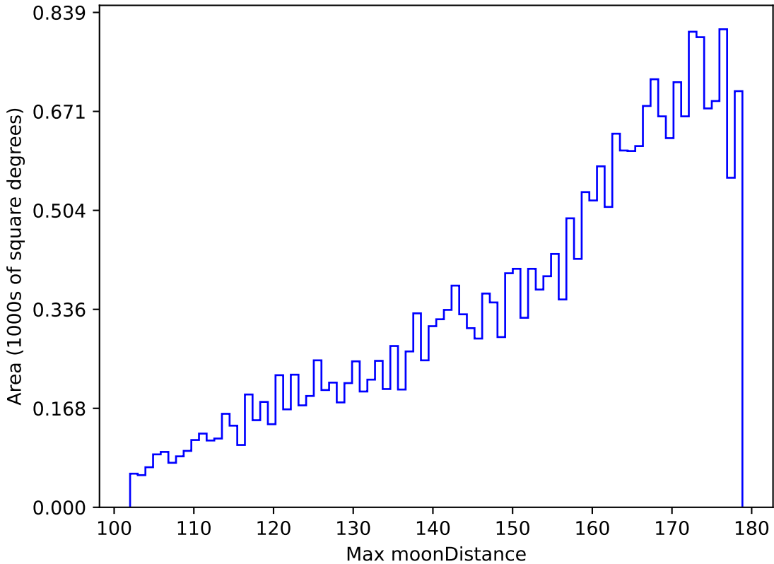
weather_cloudso0v3.4_10yrs All sky z band: Max moonDistance
