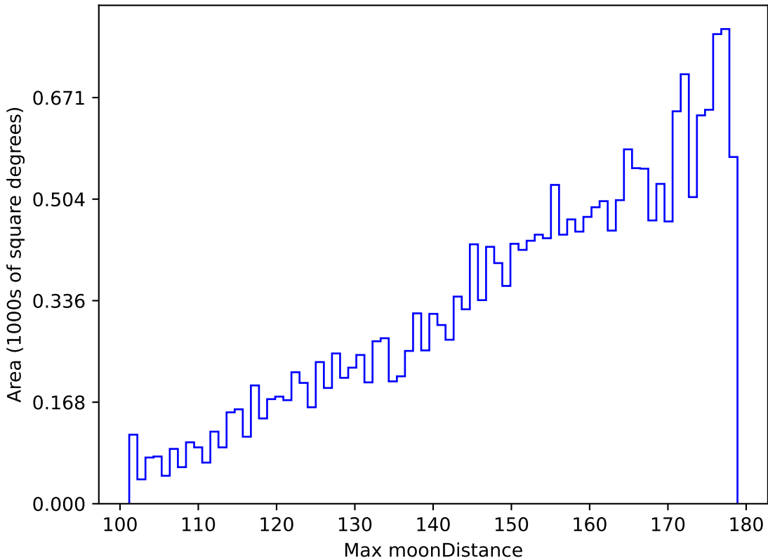
weather_cloudso0v3.4_10yrs All sky u band: Max moonDistance
