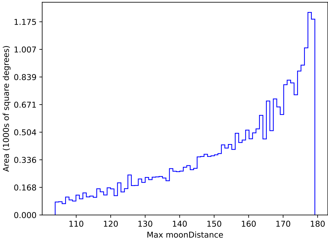
weather_cloudso0v3.4_10yrs All sky r band: Max moonDistance
