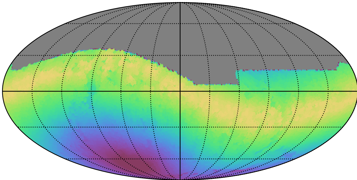
weather_cloudso0v3.4_10yrs All sky i band: Max moonDistance
