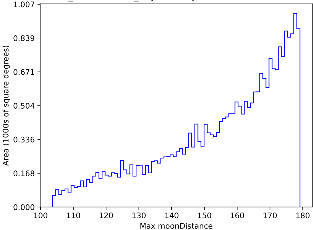
weather_cloudso0v3.4_10yrs All sky i band: Max moonDistance
