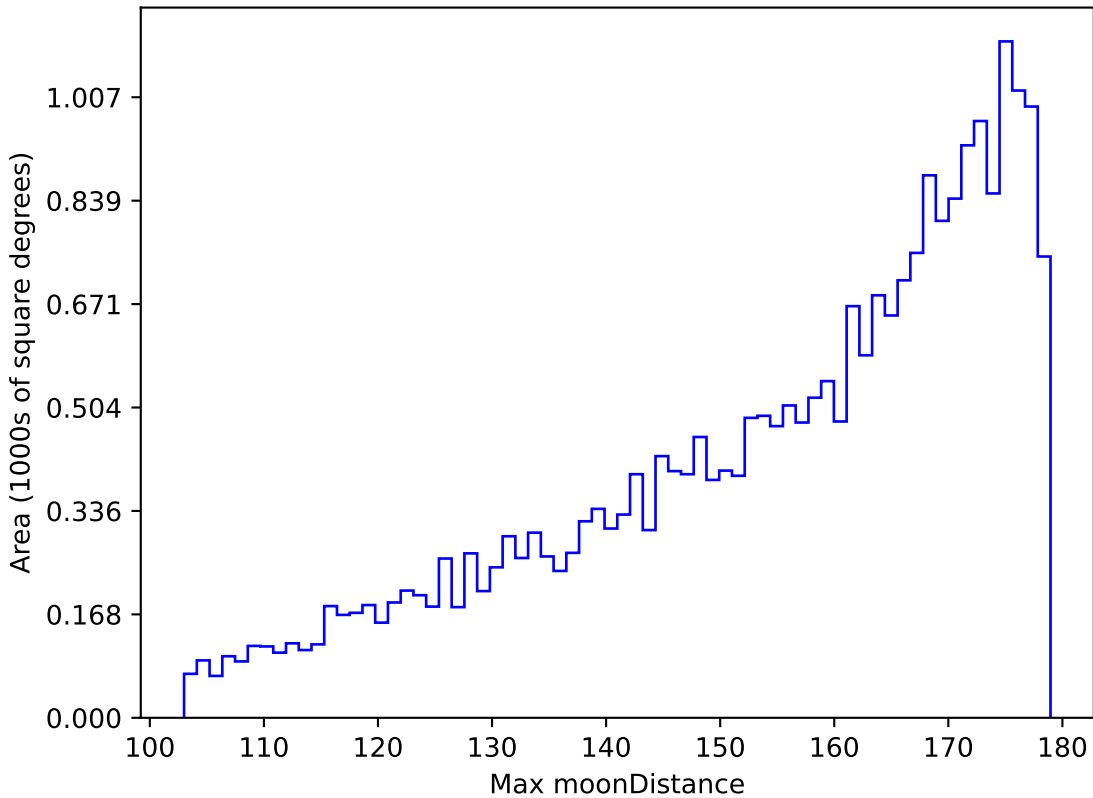
weather_cloudso0v3.4_10yrs All sky g band: Max moonDistance
