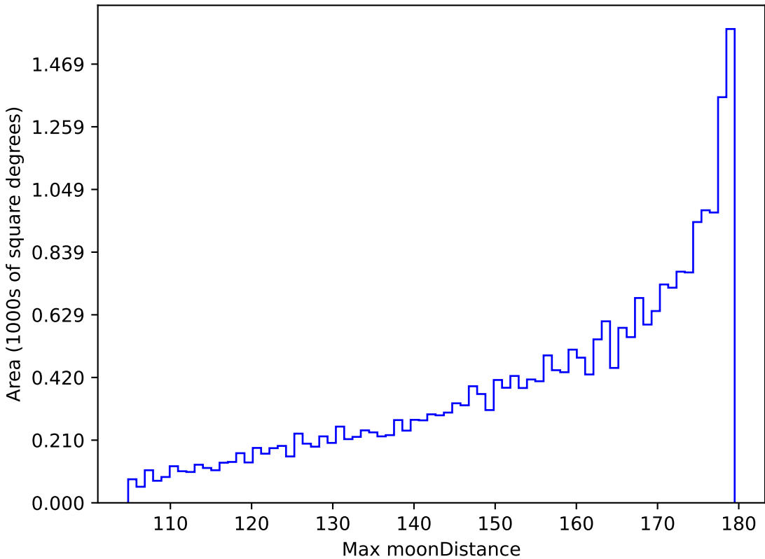
weather_cloudso0v3.4_10yrs All sky all bands: Max moonDistance
