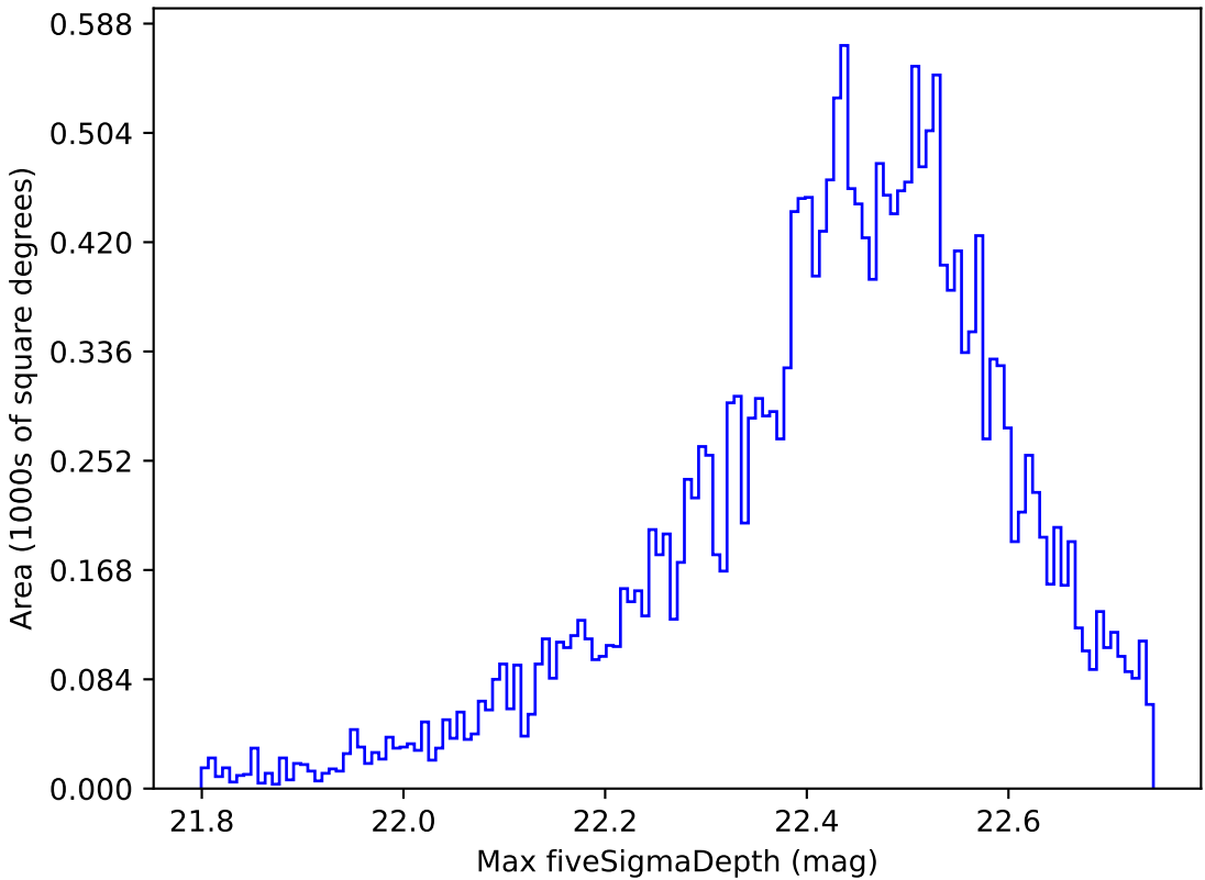
weather_cloudso0v3.4_10yrs Yr 1 y band: Max fiveSigmaDepth
