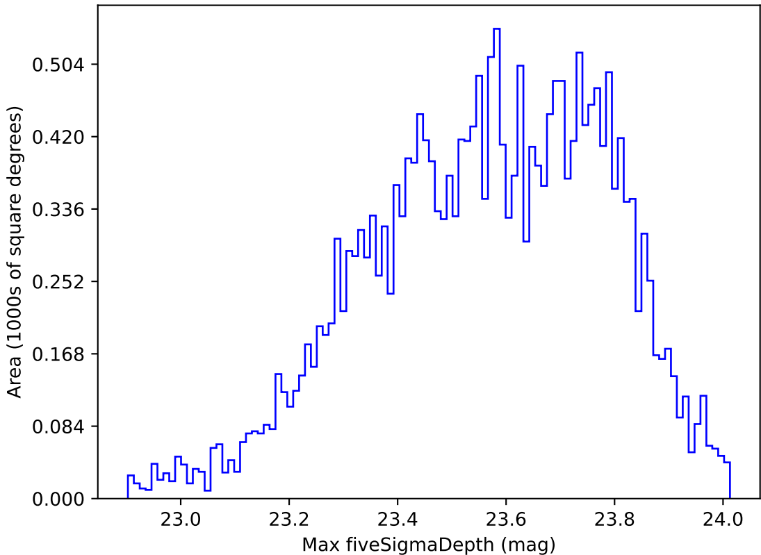
weather_cloudso0v3.4_10yrs Yr 1 u band: Max fiveSigmaDepth
