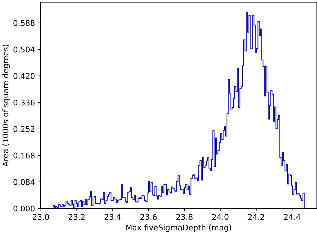
weather_cloudso0v3.4_10yrs Yr 1 i band: Max fiveSigmaDepth
