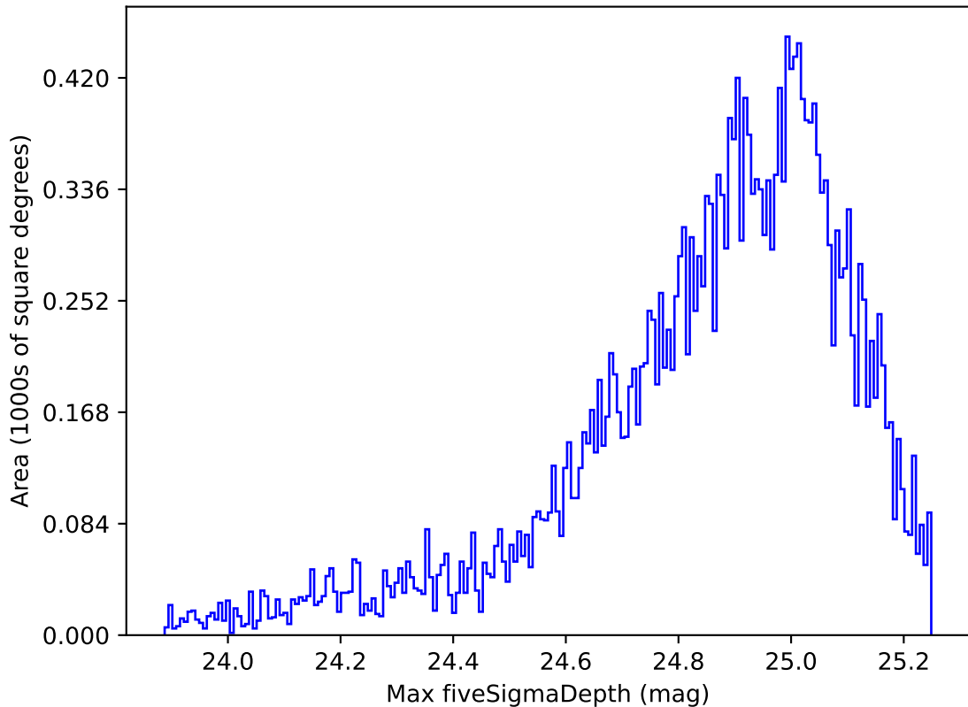
weather_cloudso0v3.4_10yrs Yr 1 all bands: Max fiveSigmaDepth
