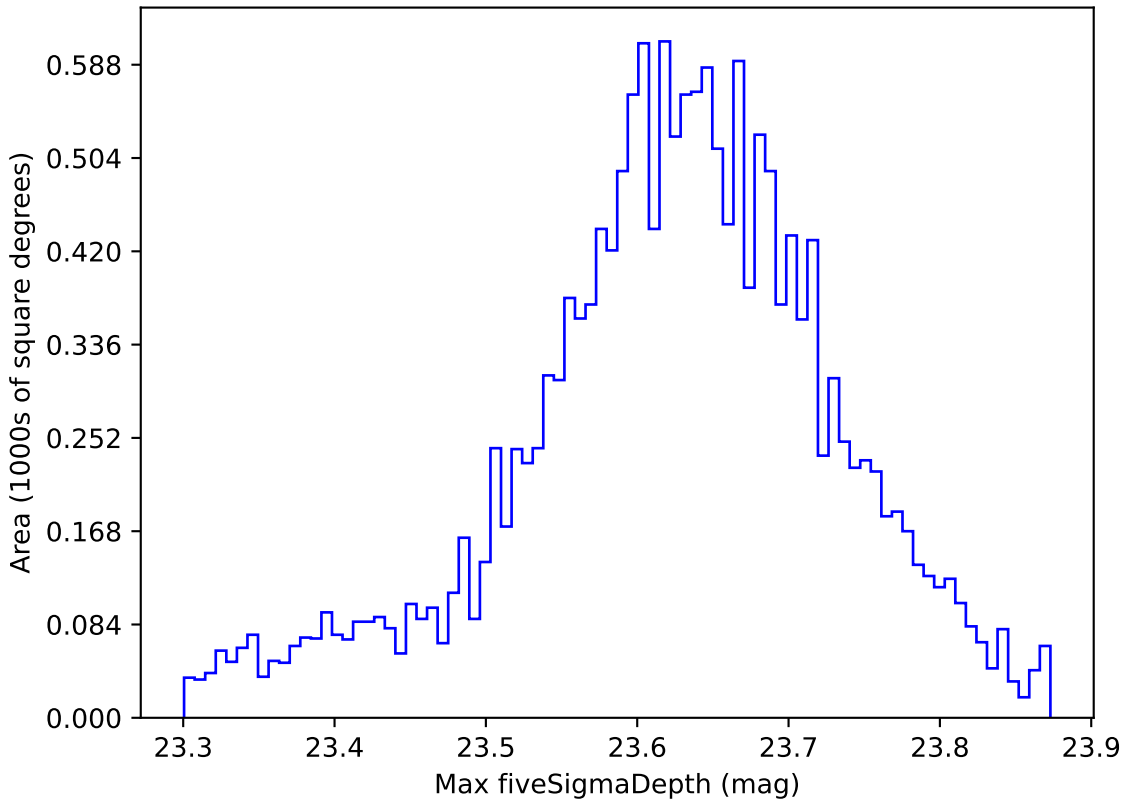
weather_cloudso0v3.4_10yrs WFD z band: Max fiveSigmaDepth
