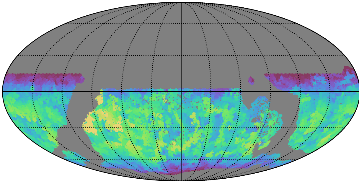
weather_cloudso0v3.4_10yrs WFD y band: Max fiveSigmaDepth
