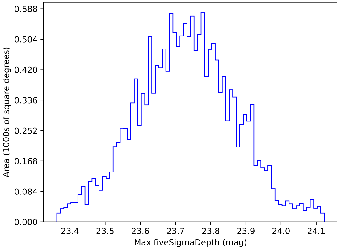
weather_cloudso0v3.4_10yrs WFD u band: Max fiveSigmaDepth
