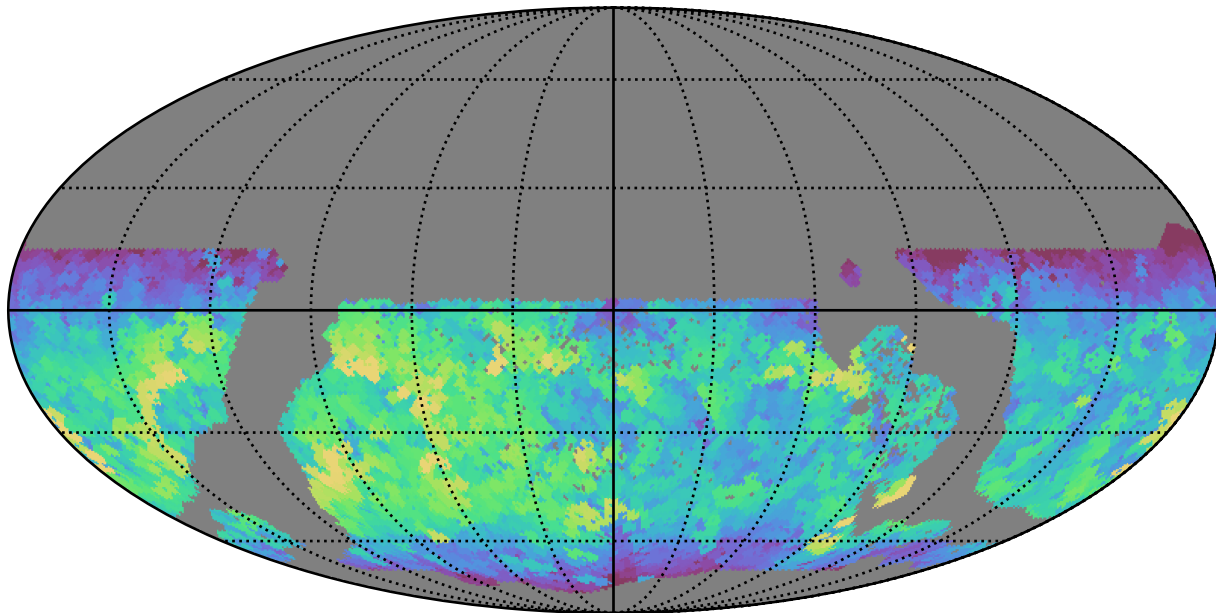
weather_cloudso0v3.4_10yrs WFD i band: Max fiveSigmaDepth
