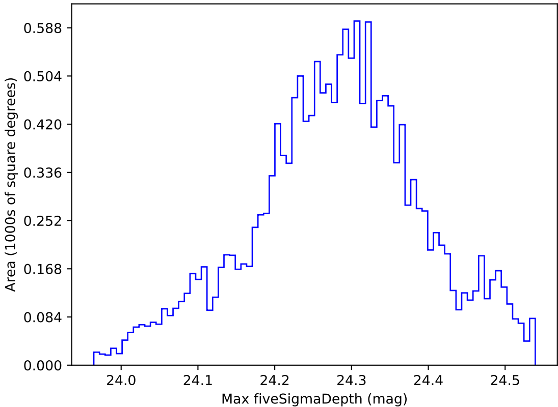
weather_cloudso0v3.4_10yrs WFD i band: Max fiveSigmaDepth
