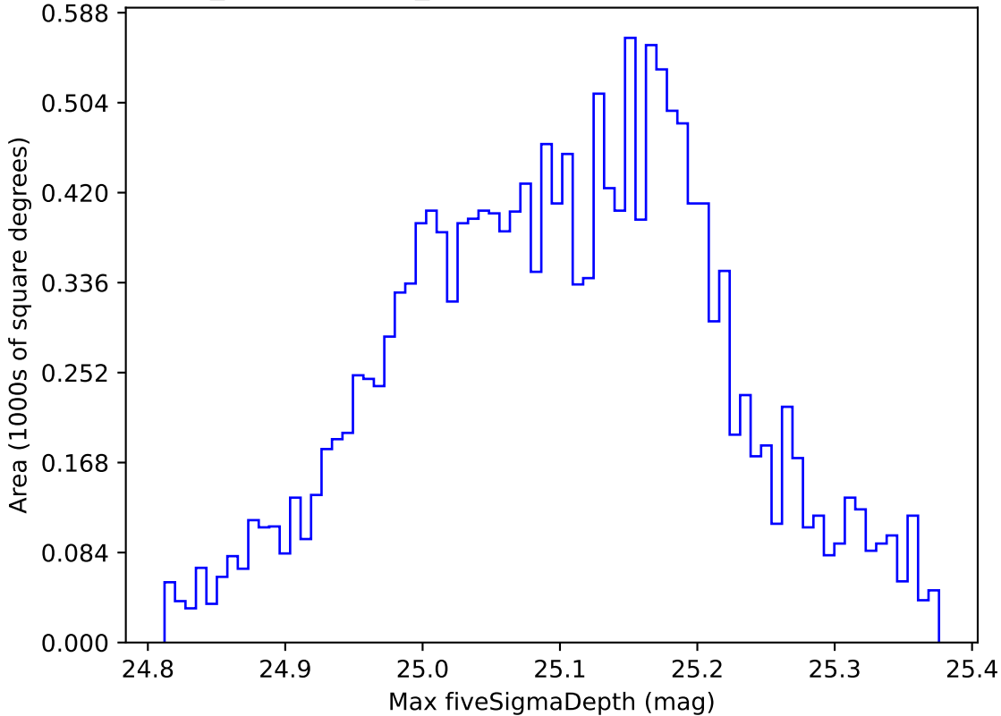
weather_cloudso0v3.4_10yrs WFD g band: Max fiveSigmaDepth
