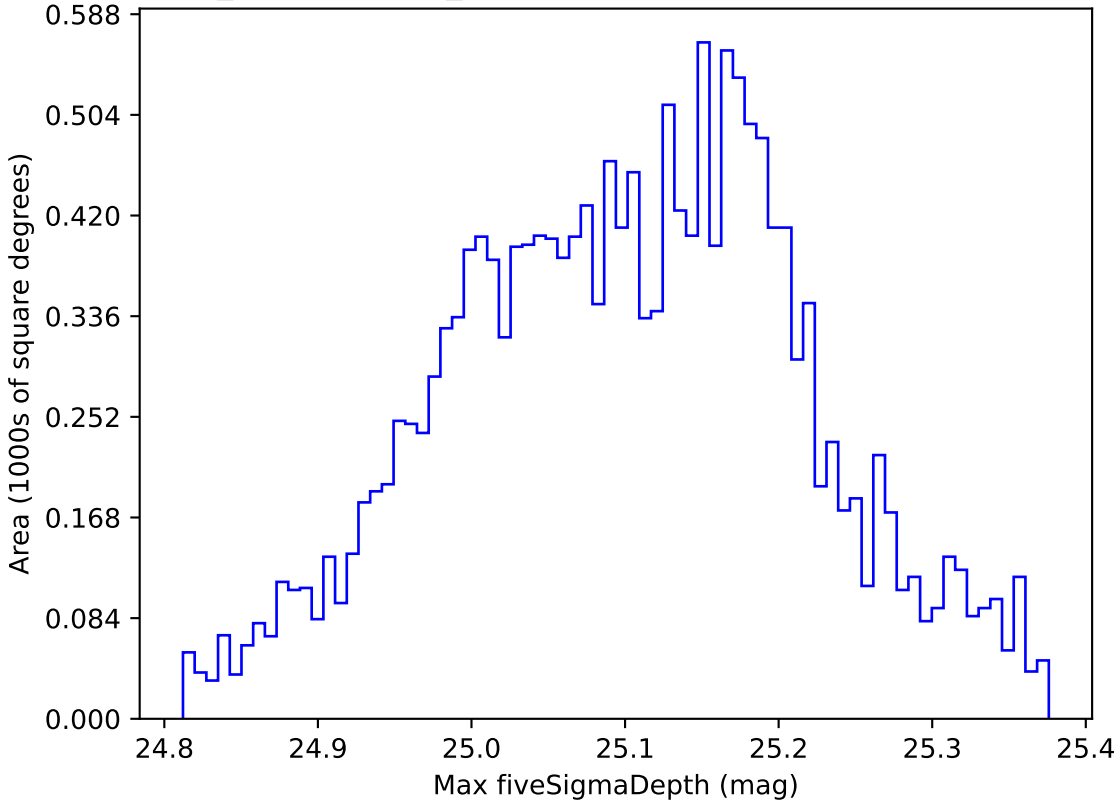
weather_cloudso0v3.4_10yrs WFD all bands: Max fiveSigmaDepth
