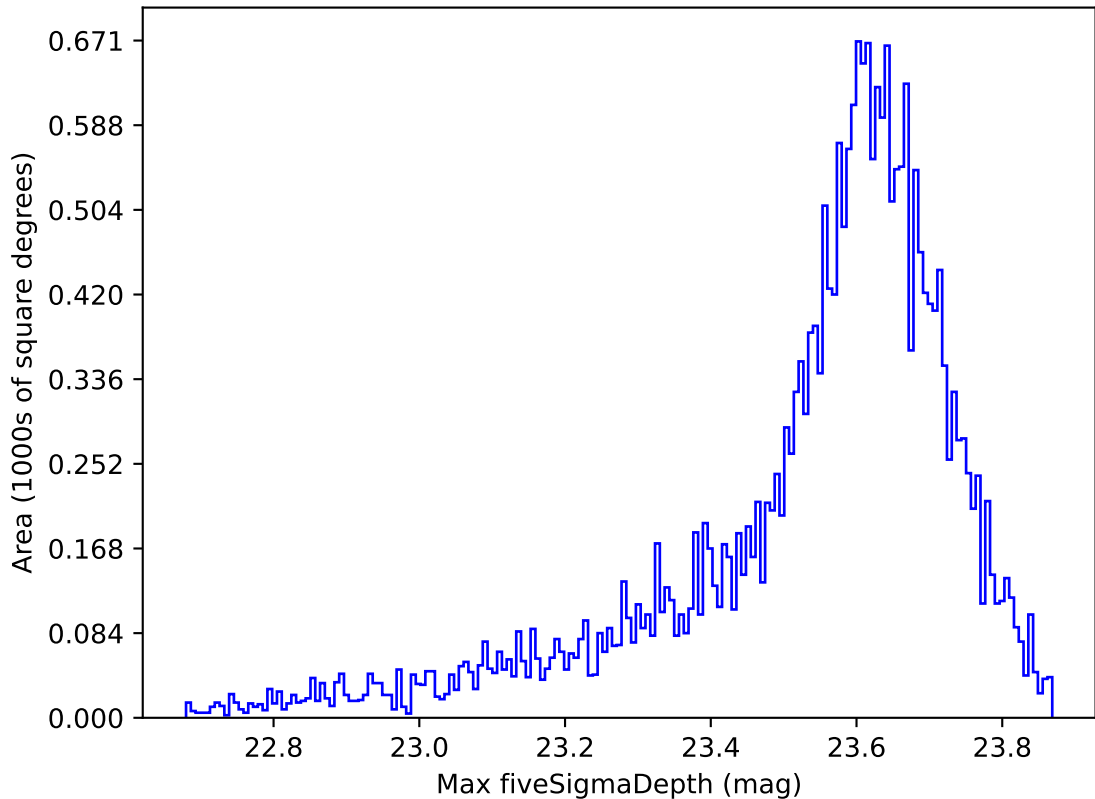
weather_cloudso0v3.4_10yrs All sky z band: Max fiveSigmaDepth
