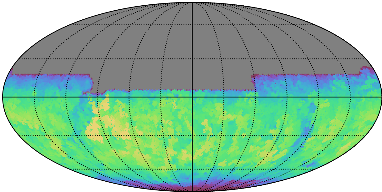
weather_cloudso0v3.4_10yrs All sky y band: Max fiveSigmaDepth
