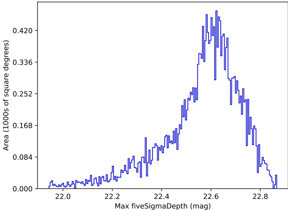
weather_cloudso0v3.4_10yrs All sky y band: Max fiveSigmaDepth
