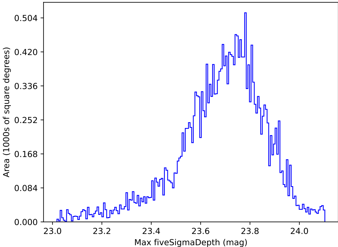
weather_cloudso0v3.4_10yrs All sky u band: Max fiveSigmaDepth
