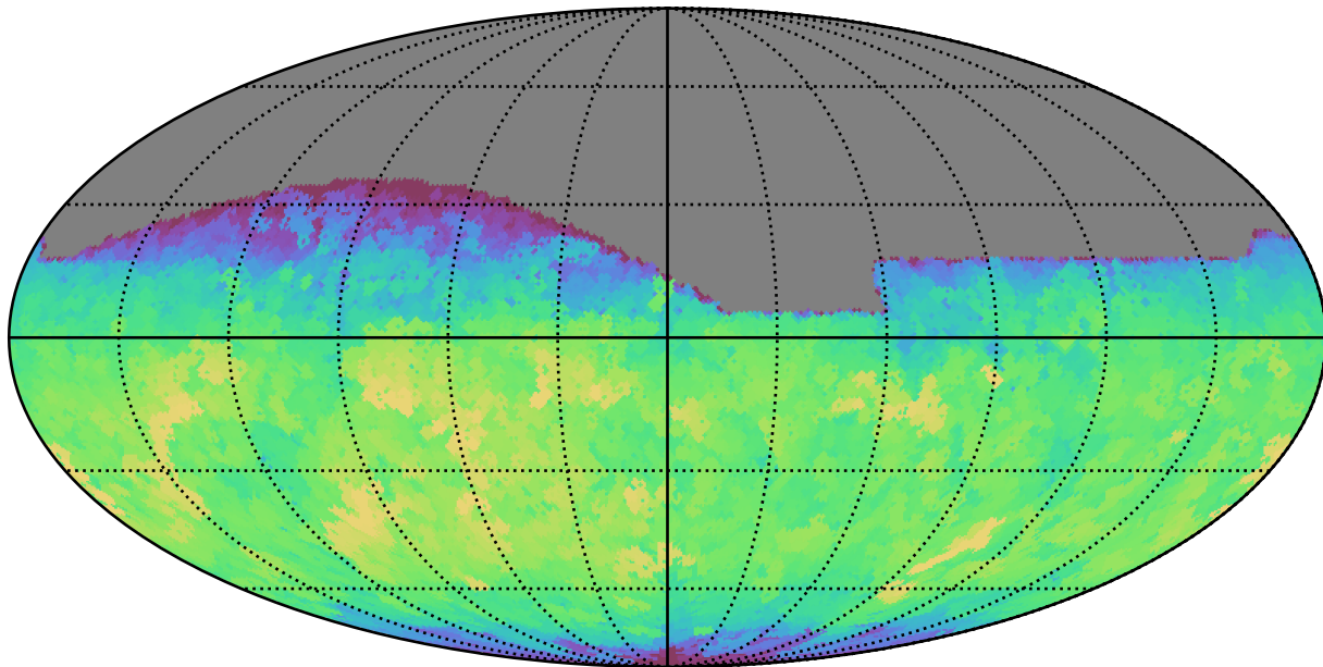
weather_cloudso0v3.4_10yrs All sky i band: Max fiveSigmaDepth
