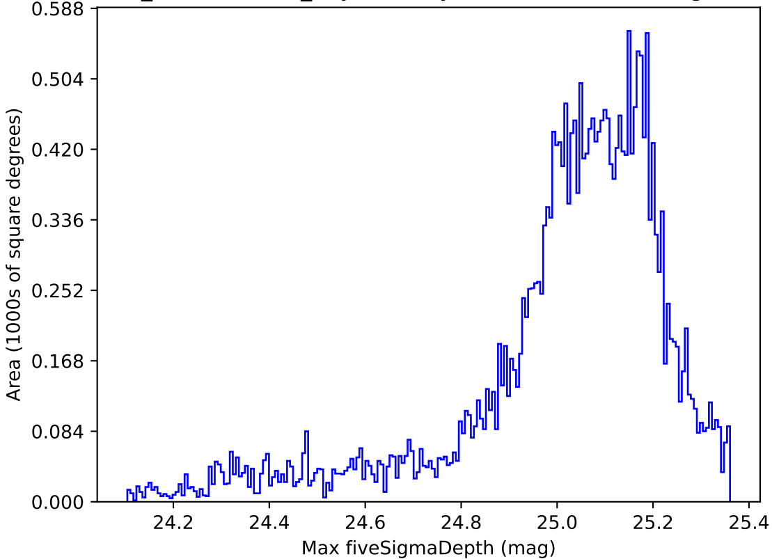
weather_cloudso0v3.4_10yrs All sky all bands: Max fiveSigmaDepth
