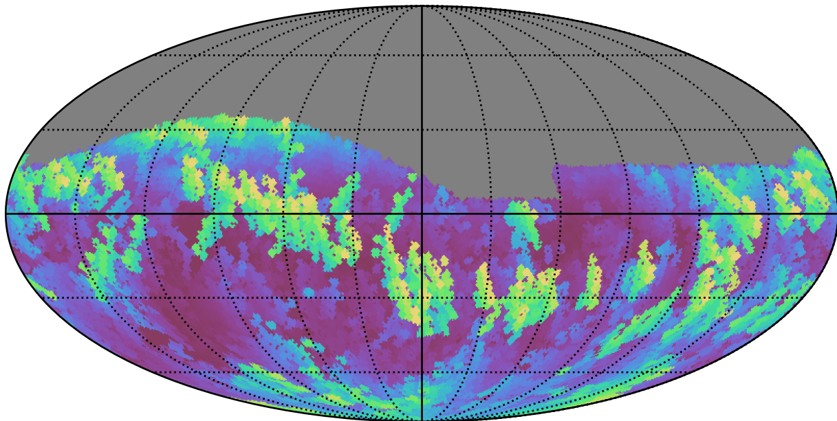
weather_cloudso0v3.4_10yrs Yr 1 z band: Max airmass
