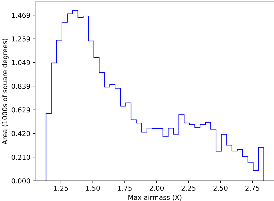
weather_cloudso0v3.4_10yrs Yr 1 z band: Max airmass
