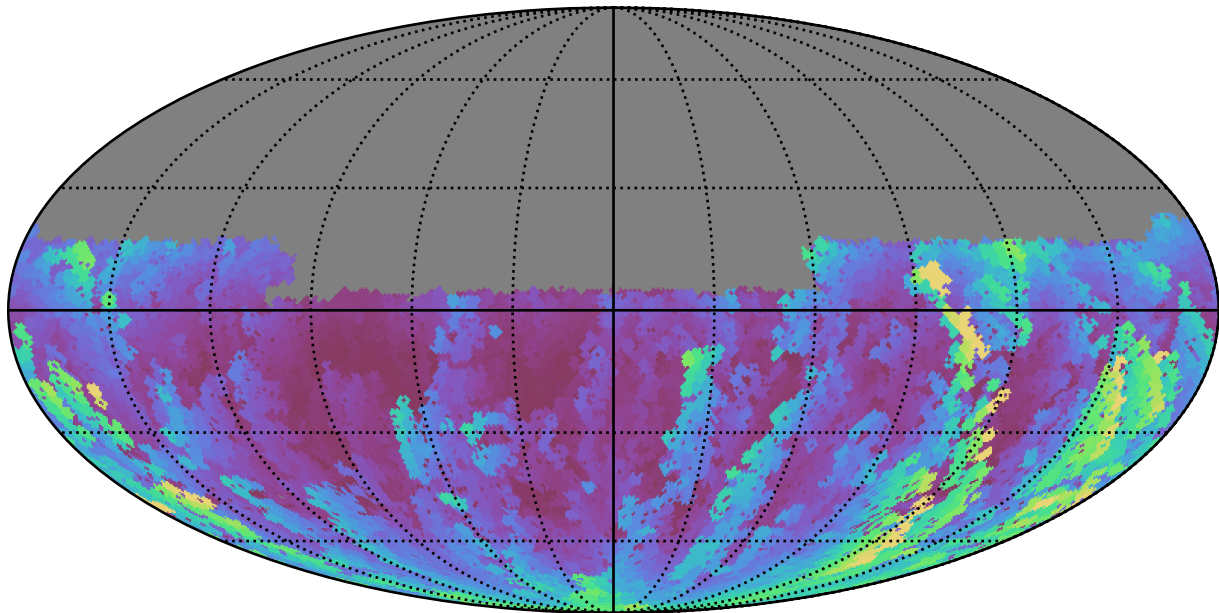
weather_cloudso0v3.4_10yrs Yr 1 u band: Max airmass
