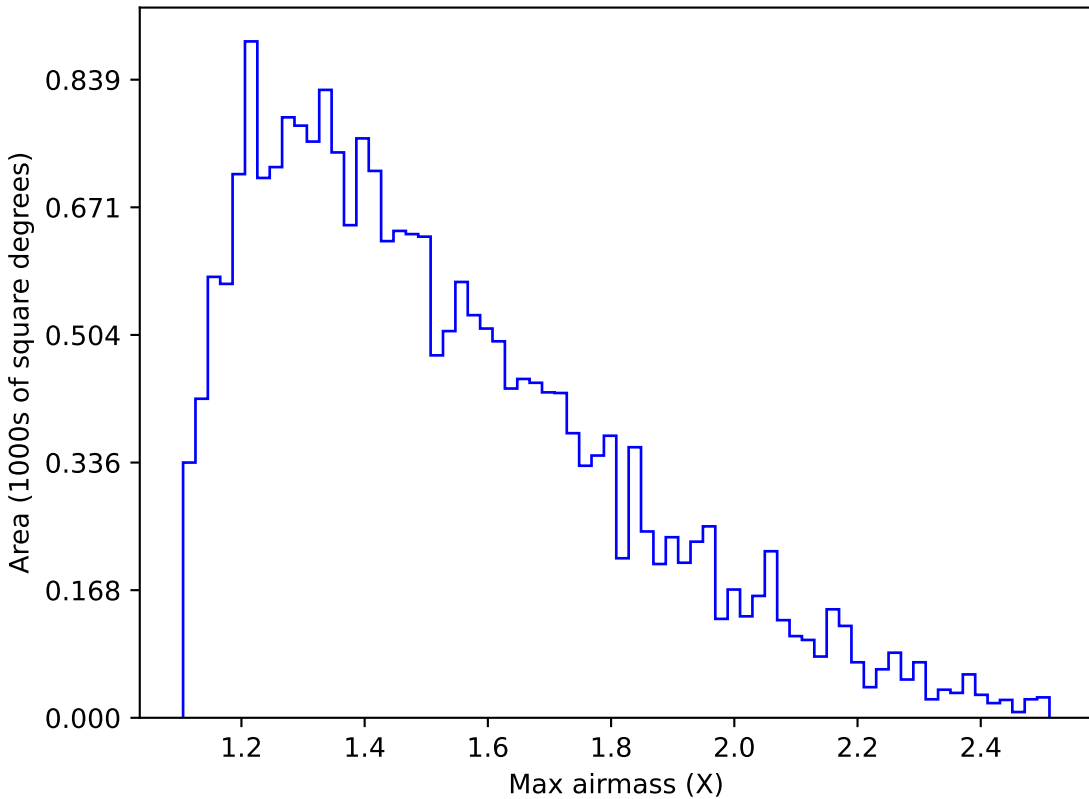
weather_cloudso0v3.4_10yrs Yr 1 u band: Max airmass
