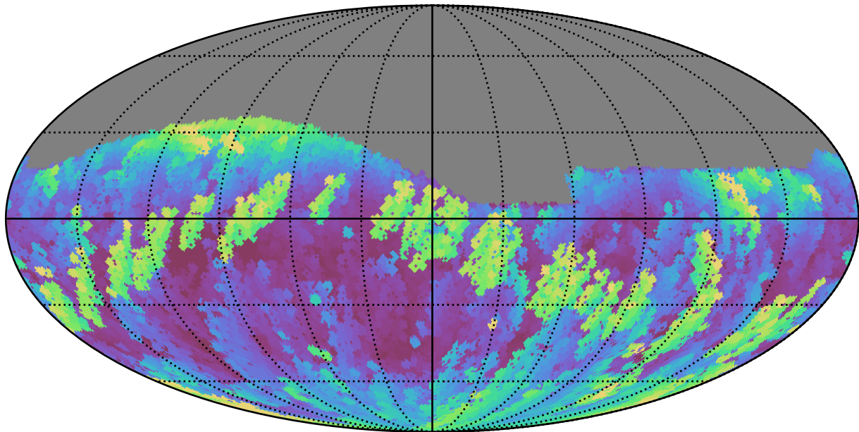
weather_cloudso0v3.4_10yrs Yr 1 r band: Max airmass
