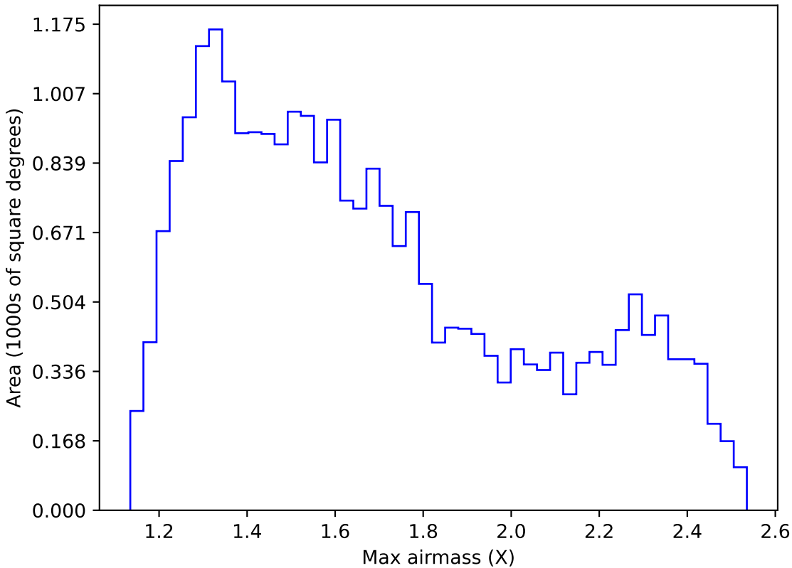
weather_cloudso0v3.4_10yrs Yr 1 r band: Max airmass
