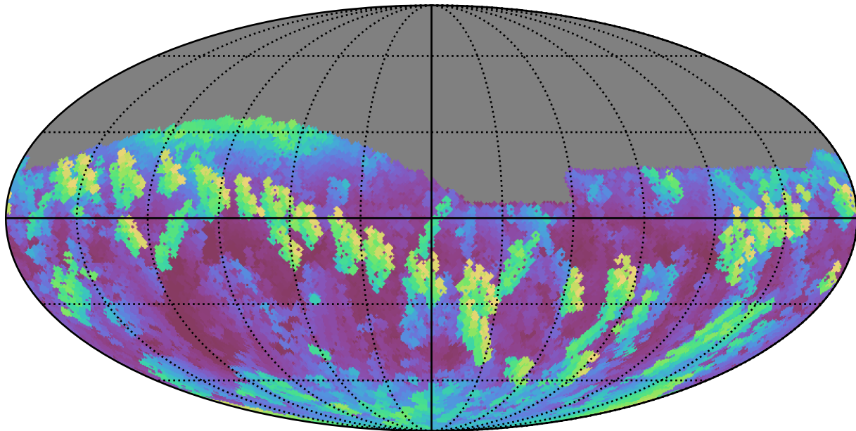
weather_cloudso0v3.4_10yrs Yr 1 i band: Max airmass
