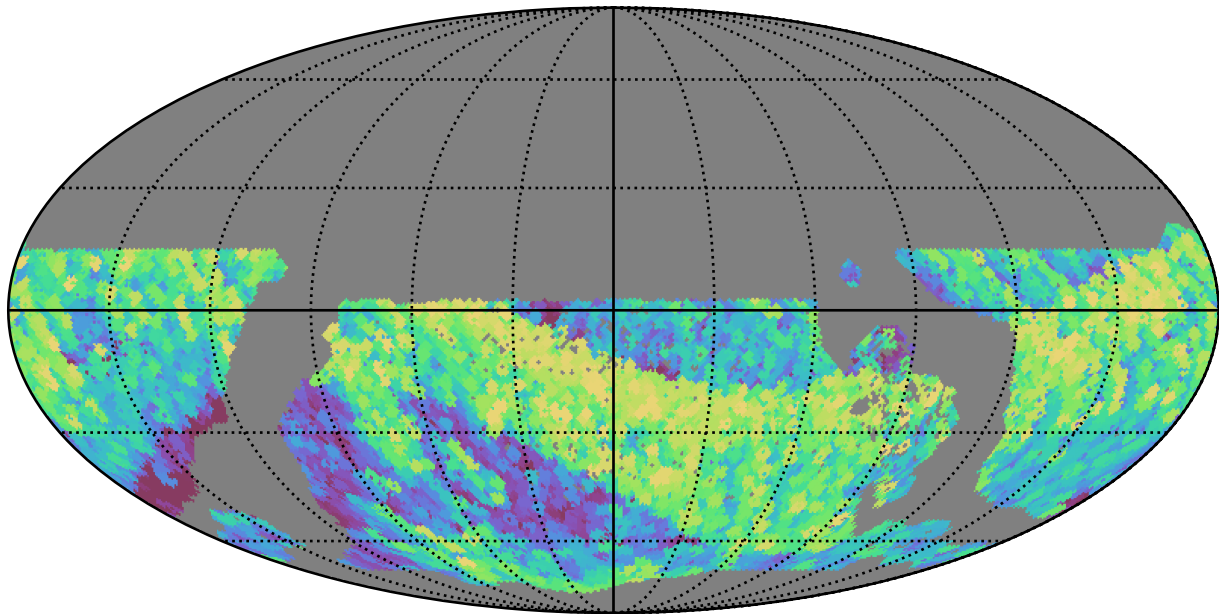
weather_cloudso0v3.4_10yrs WFD z band: Max airmass
