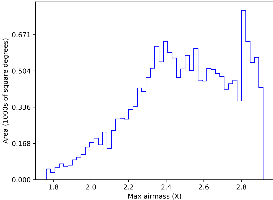
weather_cloudso0v3.4_10yrs WFD z band: Max airmass
