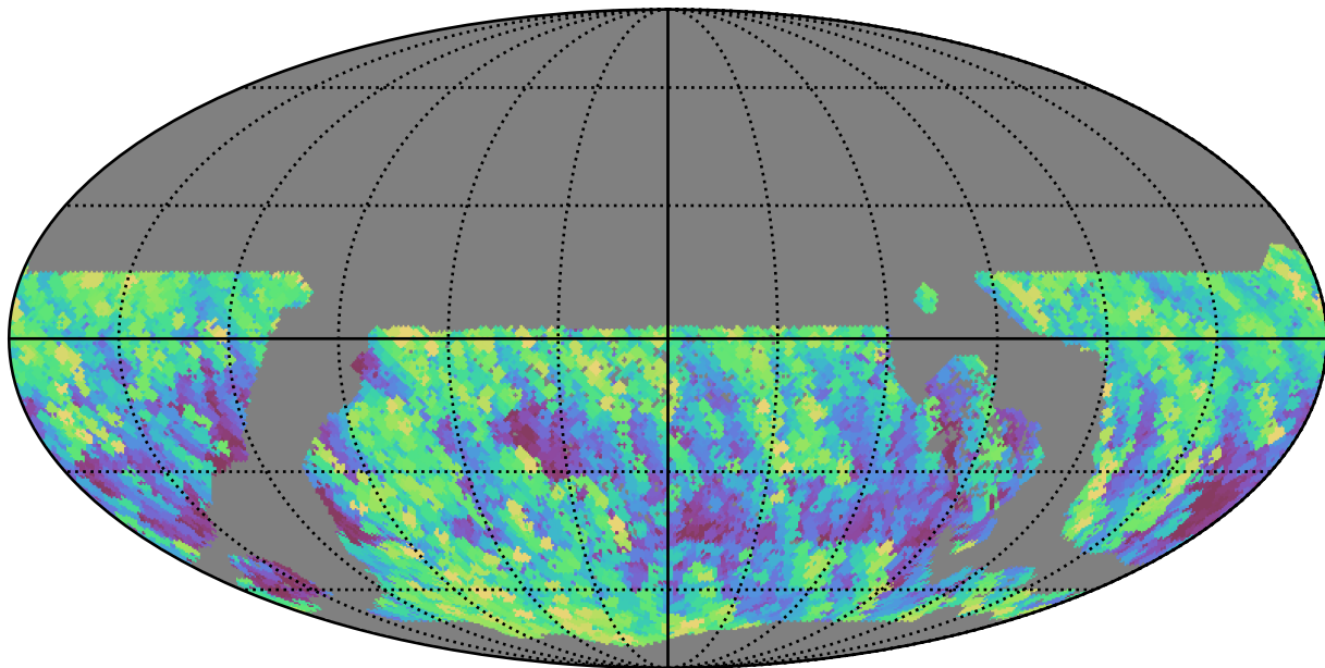
weather_cloudso0v3.4_10yrs WFD y band: Max airmass
