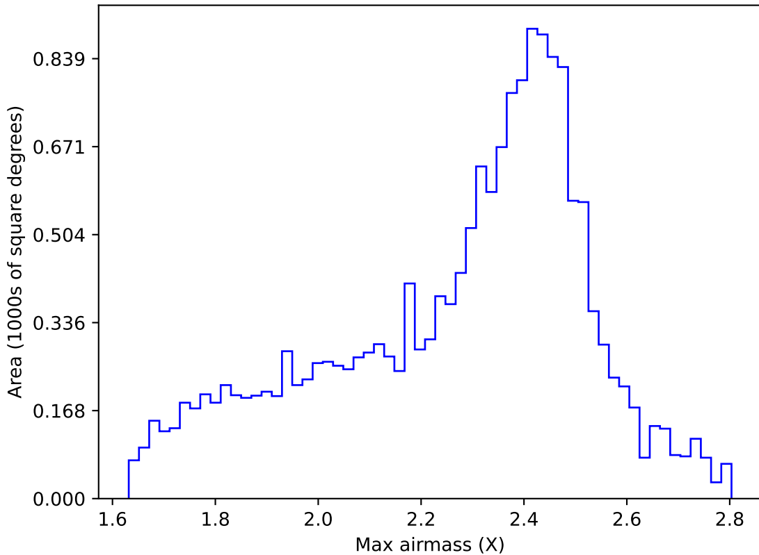
weather_cloudso0v3.4_10yrs WFD r band: Max airmass
