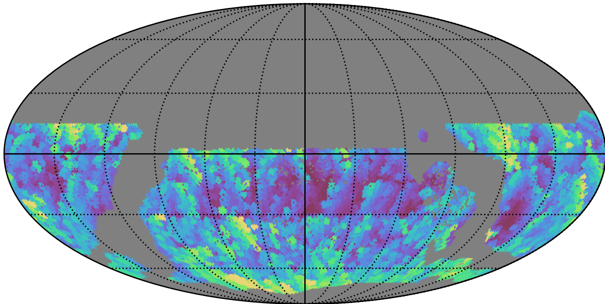
weather_cloudso0v3.4_10yrs WFD g band: Max airmass
