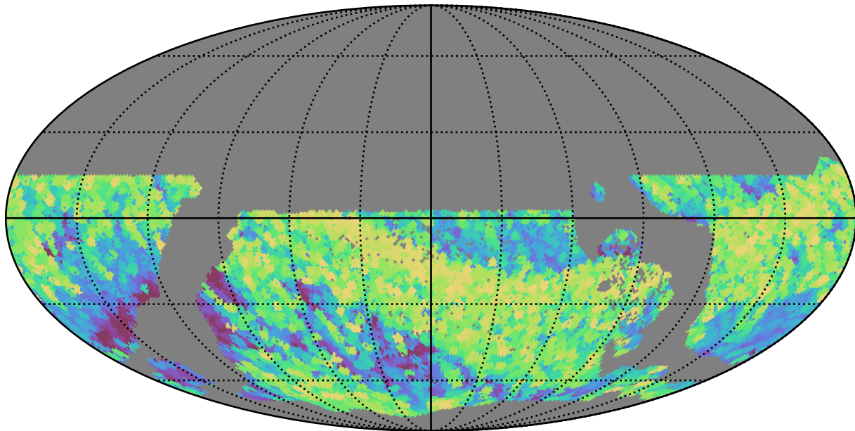
weather_cloudso0v3.4_10yrs WFD all bands: Max airmass
