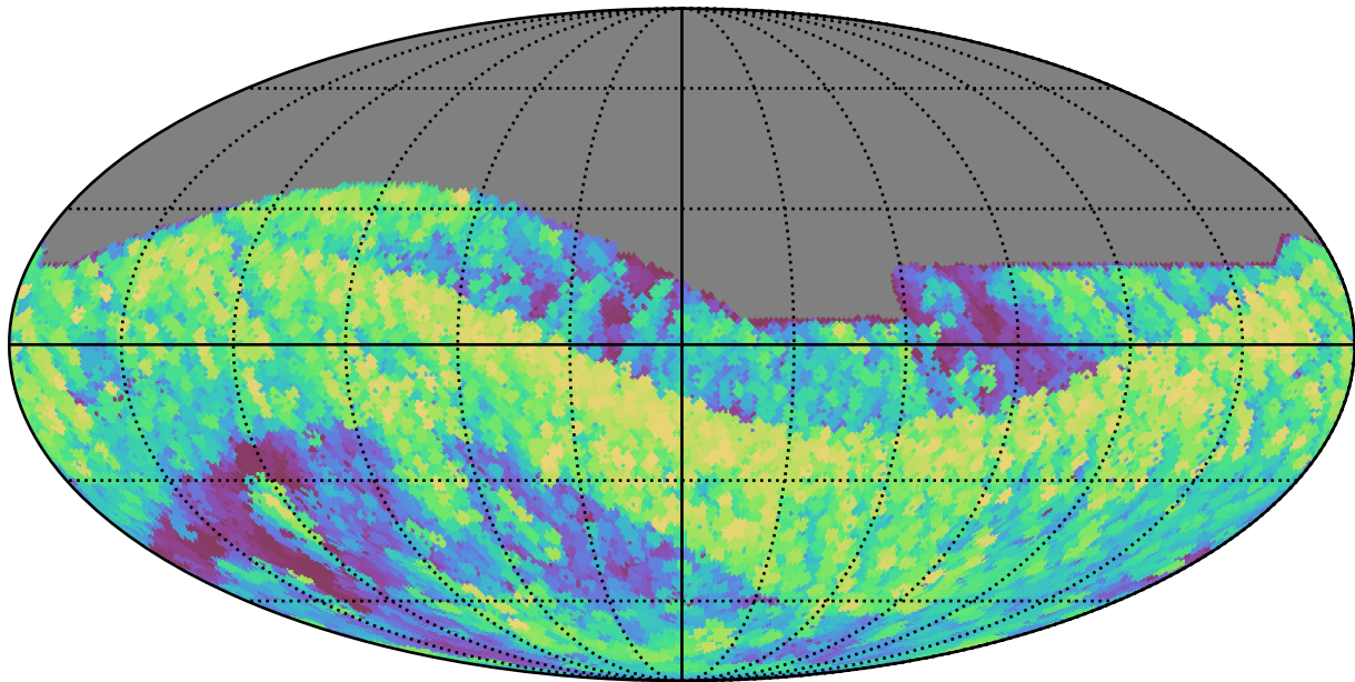
weather_cloudso0v3.4_10yrs All sky z band: Max airmass
