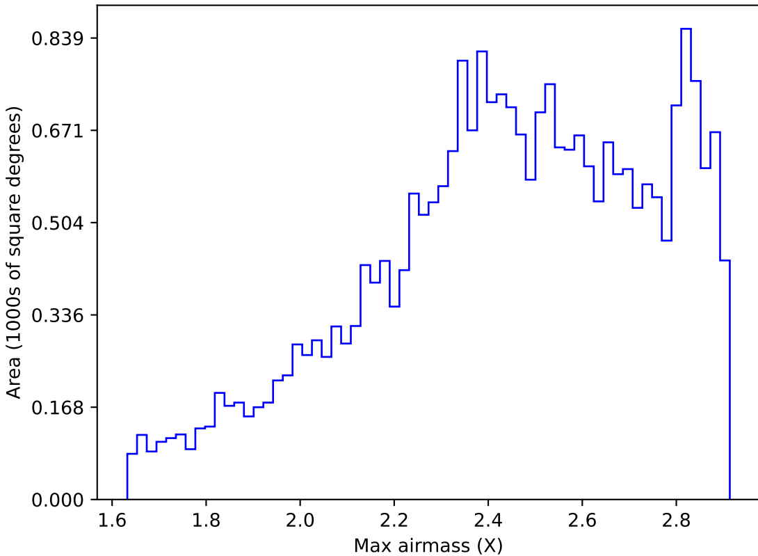
weather_cloudso0v3.4_10yrs All sky z band: Max airmass
