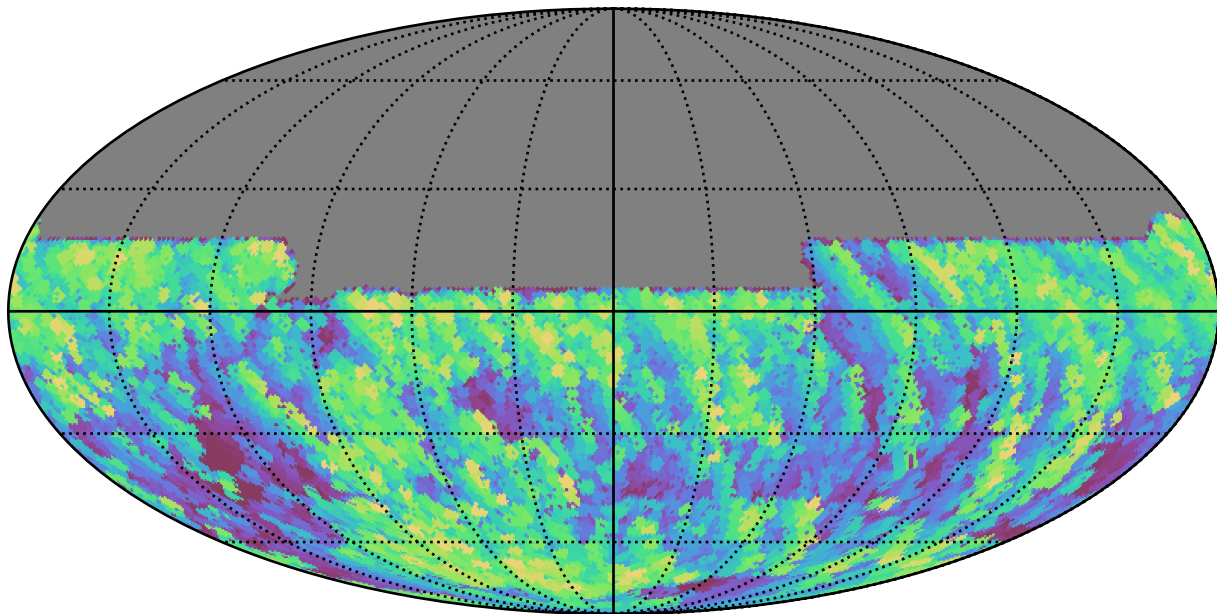
weather_cloudso0v3.4_10yrs All sky y band: Max airmass
