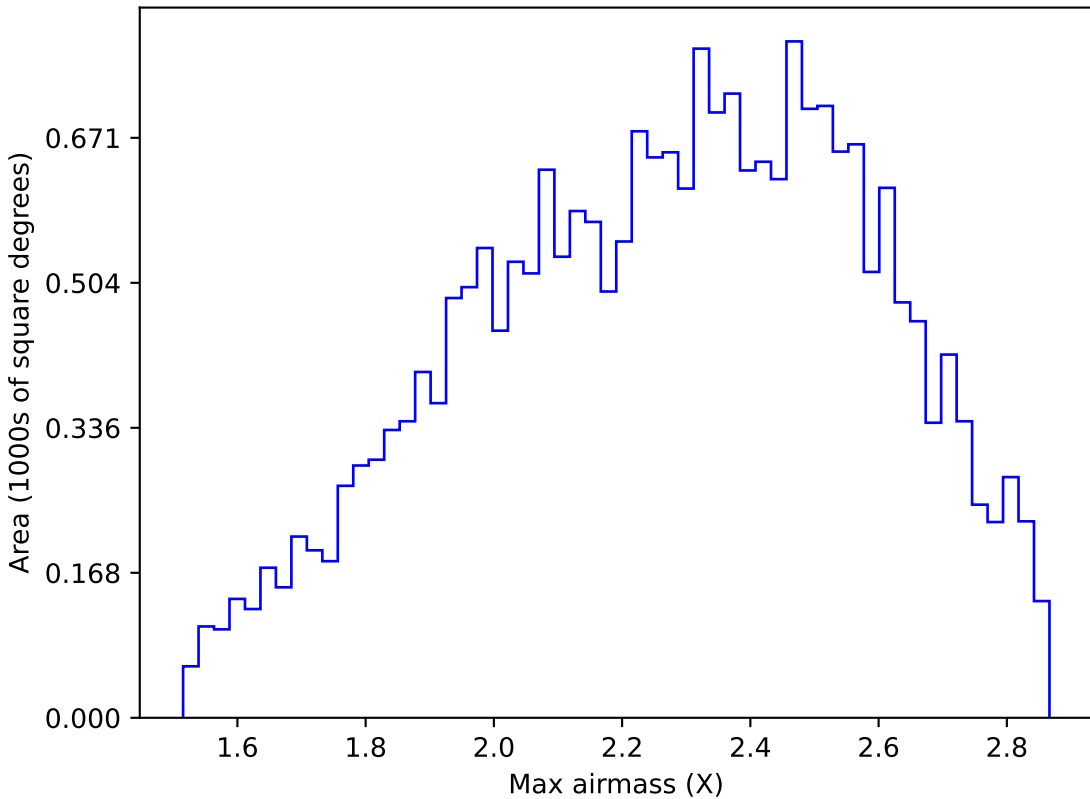
weather_cloudso0v3.4_10yrs All sky y band: Max airmass
