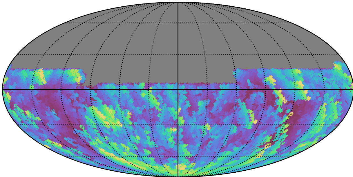
weather_cloudso0v3.4_10yrs All sky u band: Max airmass
