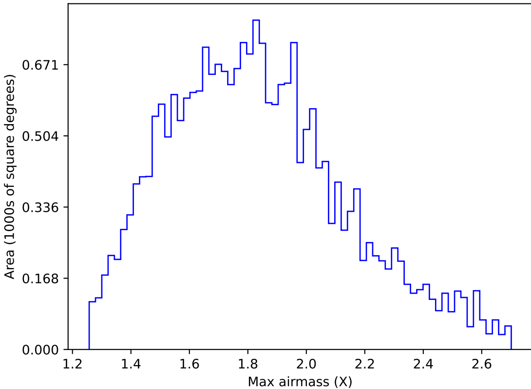
weather_cloudso0v3.4_10yrs All sky u band: Max airmass
