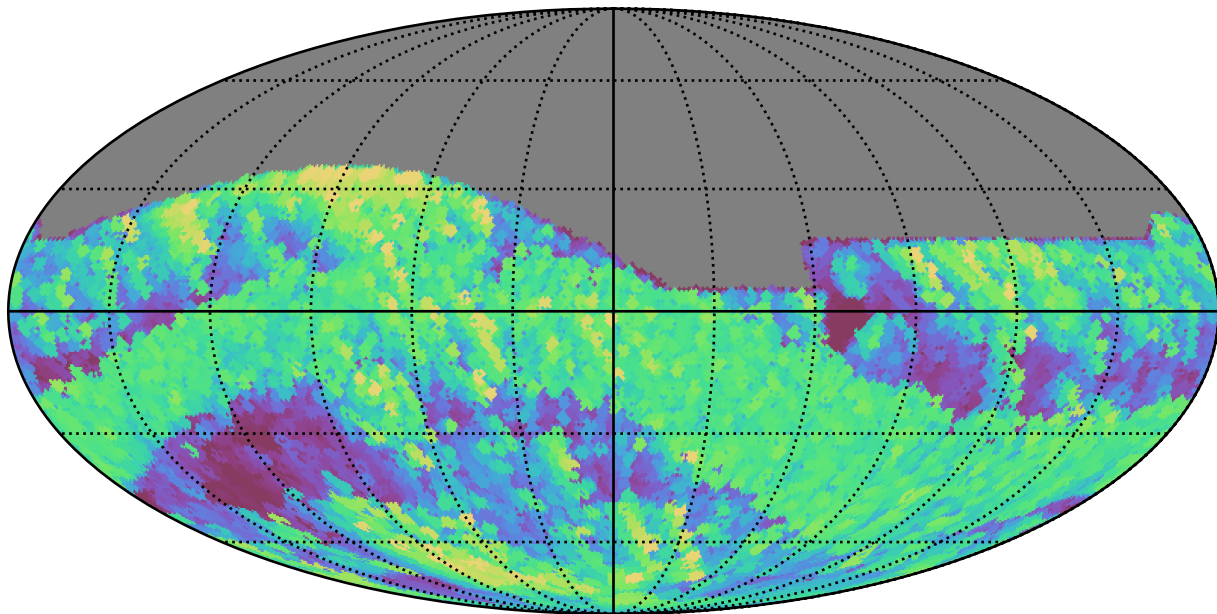
weather_cloudso0v3.4_10yrs All sky r band: Max airmass
