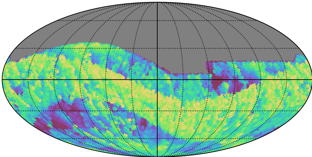
weather_cloudso0v3.4_10yrs All sky i band: Max airmass
